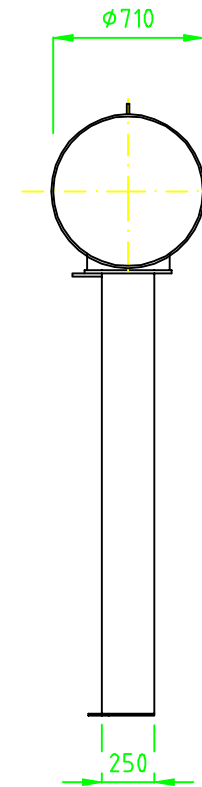
FRONT VIEW
