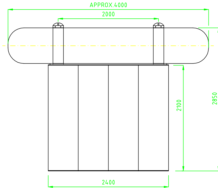
SIDE VIEW
